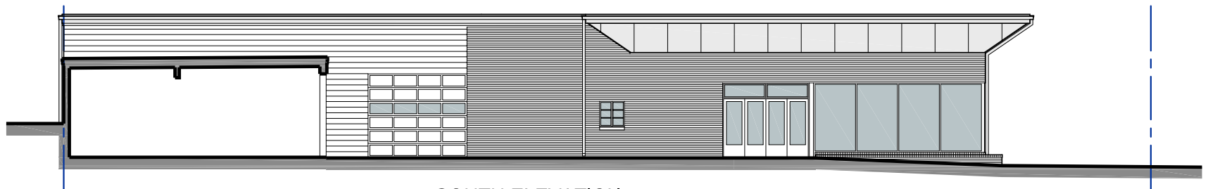
SOUTH ELEVATION
