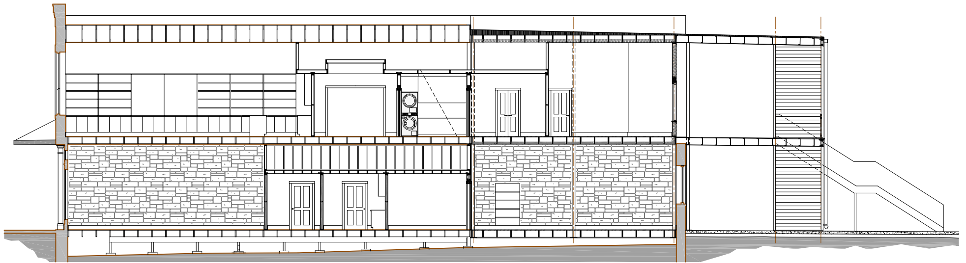
SECTION 1
