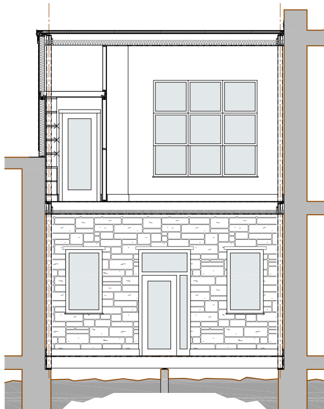
SECTION 2
