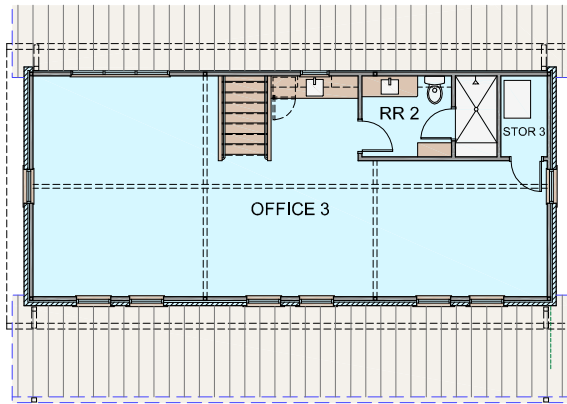
SECOND FLOOR 928 SF
