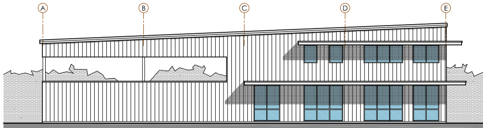
SIDE ELEVATION
