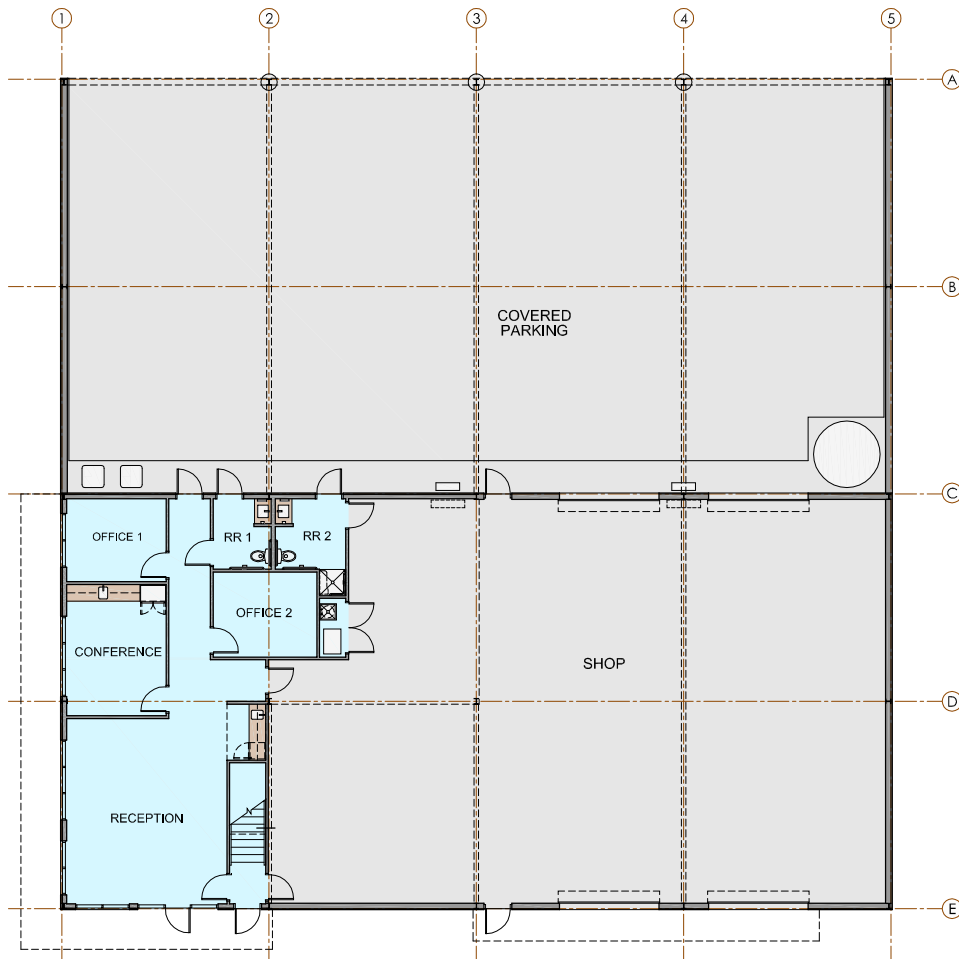
FIRST FLOOR
