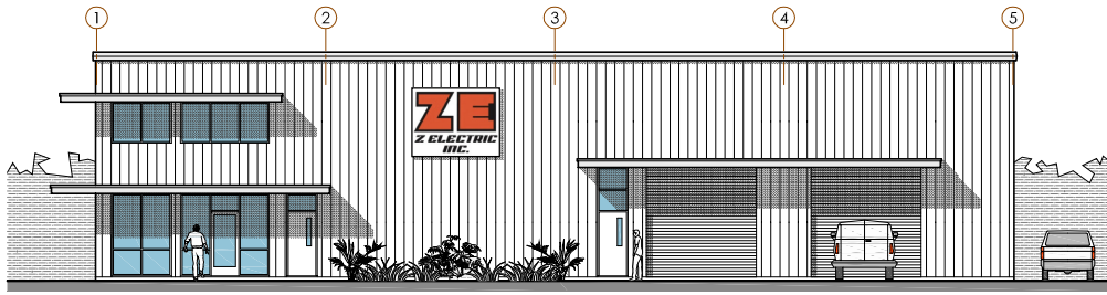
FRONT ELEVATION
